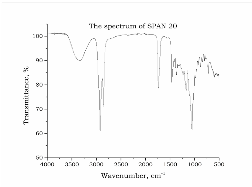
Figure S5. The spectrum of SPAN 20
