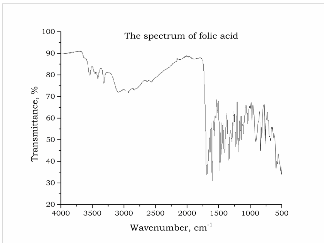
Figure S1. The spectrum of folic acid
