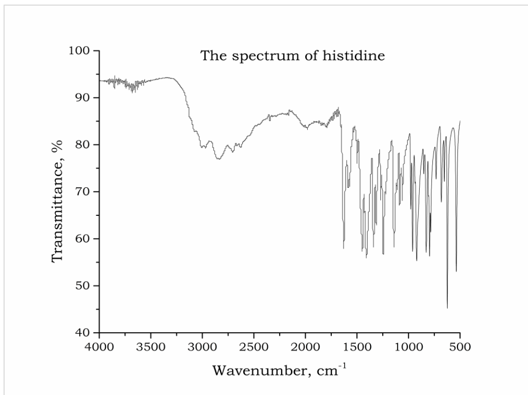
Figure S2. The spectrum of histidine
