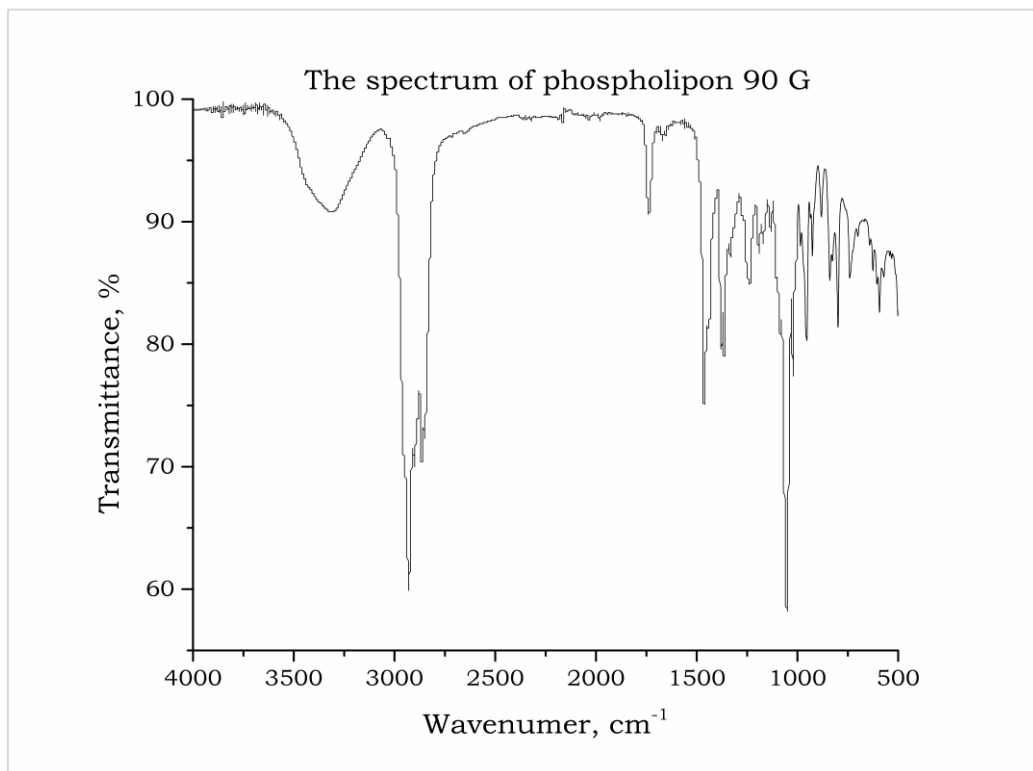
Figure S3. The spectrum of phospholipon 90 G
