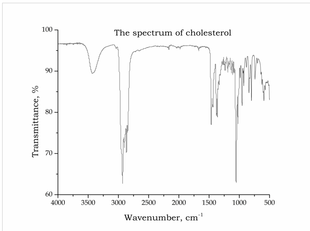
Figure S4. The spectrum of cholesterol
