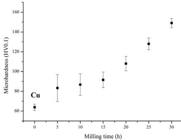
Fig. 3. Changing of microhardness values during milling time.
