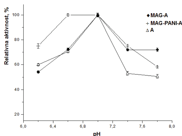
Slika 7. Uticaj pH na aktivnost native i imobilisane \alpha -amilaze. Figure 7. The effect of pH on the activity of native and immobilized \alpha -amylase.
