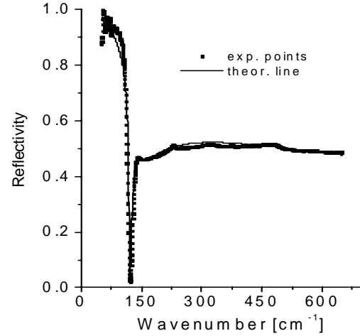
Fig. 2. Far infrared spectrum of PbTe doped with 0.2at%Fe as a function of the wavenumber, measured at T=110 K.
