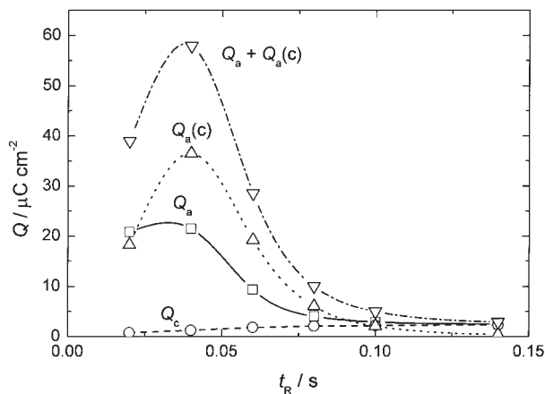
Fig. 10. Dependence of different charges, obtained by integration of the area under the corresponding j-t transients presented in Fig. 7b, as a function of the duration of the R pulse ( t_R ): Q_a represents the charge under the P pulse, anodic transient (first transient), Q_c represents the cathodic charge under the R pulse (second transient), Q_a(c) represents the anodic charge under the R pulse (second transient) and Q_a + Q_a(c) represents the total anodic charge under both the P and R pulses (first and second transient).
