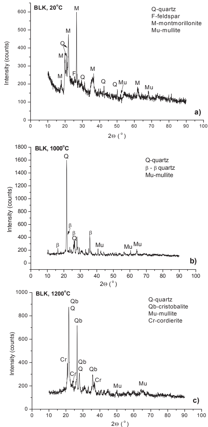
Fig. 2. XRD patterns of the fly ash-bentonite samples: a) at ambient temperature, b) after sintering at 1000 °C, and c) after sintering at 1200 °C.
