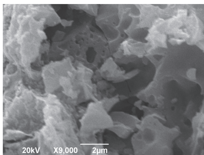
Fig. 8. SEM image of a detail of BLK sample (at ambient temperature).
