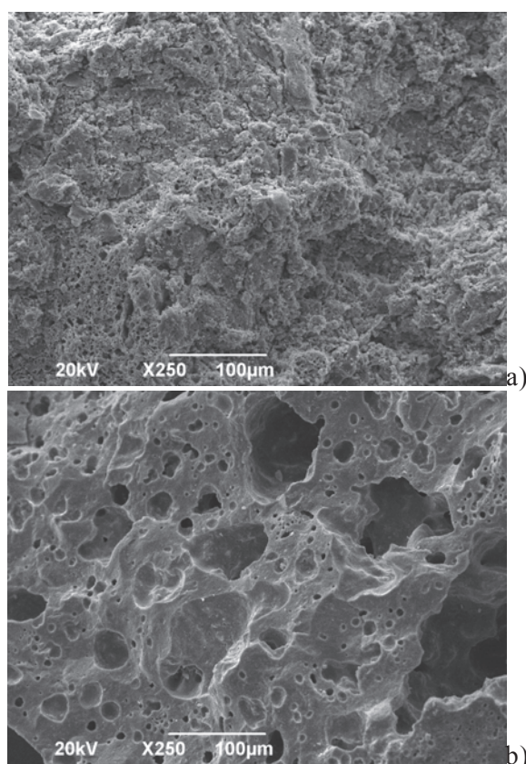
Fig. 5. SEM images of the ZLK composites: a) before sintering, b) after sintering at 1200 °C.
