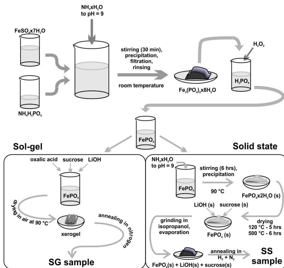
Fig.1. Schematic illustration of the synthesis processes
