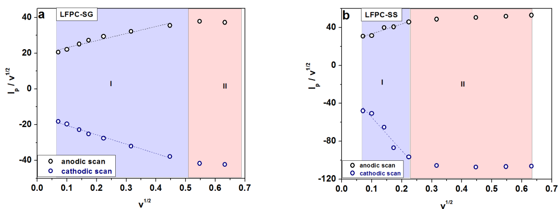
Fig.10. The dependence of I_p / v^{1/2} on v^{1/2} for SG (a) and SS(b) samples. The label v refers to the scan rate
