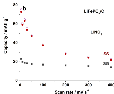
Fig.7. Comparison of the specific capacities of SS and SG samples in aqueous 6M \text{LiNO}_3 solution calculated from the voltammogram surfaces; the solid symbols relate to the intercalation and the empty symbols relate to the deintercalation.
