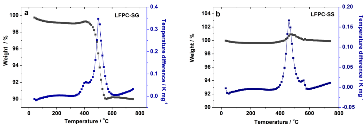
Fig. 4. The TG/DTA curves of the SG (a) and SS (b) samples under an air flow at a heating rate 10 \text{ }^\circ\text{C} .
