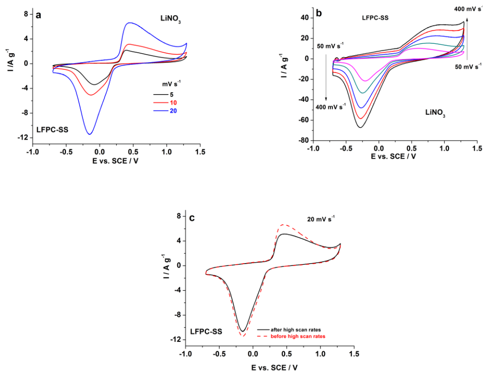
Fig.6 Cyclic voltammograms of LFPC-SS sample in aqueous 6M LiNO 3 solution at: a) low polarization rates, b) high polarization rates; c) two cycles at 20 mV s -1 with one intermediate cycle (not shown) at 400 mV s -1 .
