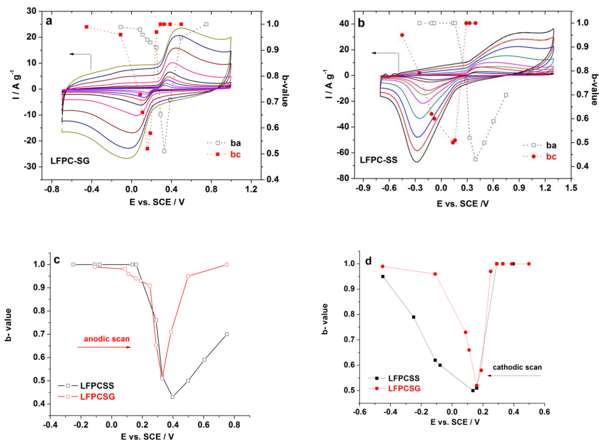
Fig.9. b-values calculated at various potentials corresponding to the lithiation/delithiation of SG (a) and SS(b) samples. The b-values for both composites were shown in a comparative way in the insets c) and d), for the anodic and cathodic scan, respectively.
