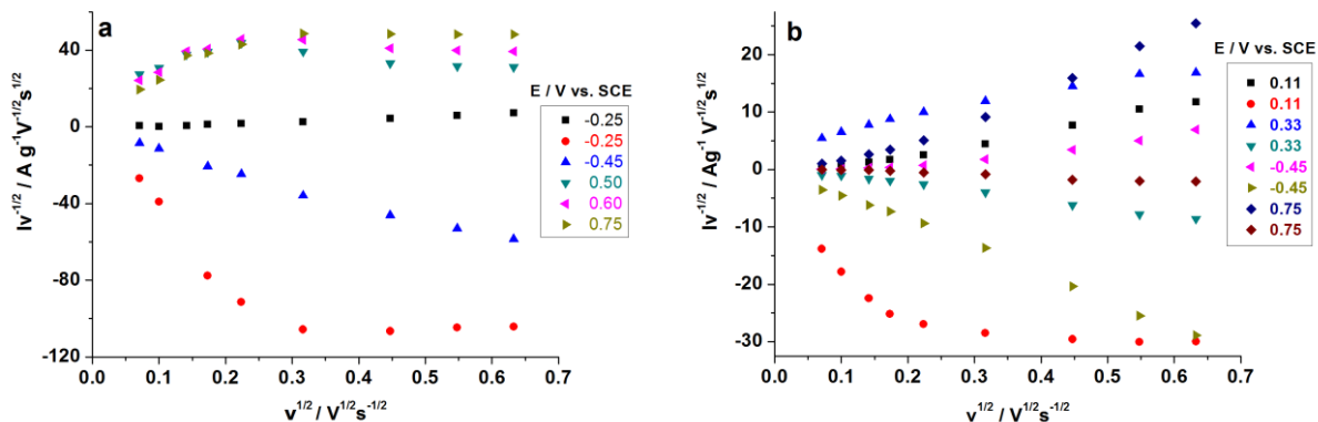
Fig. 11 The isotopotential dependence of I/v^{1/2} on v^{1/2} for SS (left) and SG(right) samples. The potentials, both lower and higher than reversible one were used to construct graphs. The potentials for each graph are marked in insets.
