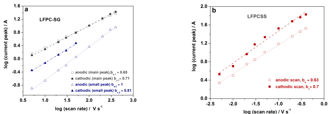
Fig. 8. log I_p - log v plot of LFPC-SG (a) and LFPC-SS whose values correspond to the main maximums of CV peaks. Their slopes against log(scan rate) axis ( b values) are marked in insets
