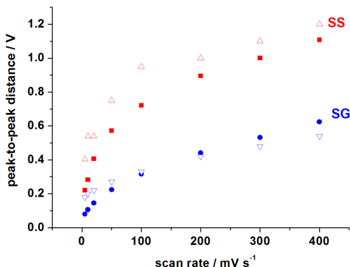
Fig.12 Peak-to-peak potential distance in function on scan rate for SS and SG samples, experimental points (empty symbols) versus those calculated by means of Eq.5 (full symbols).
