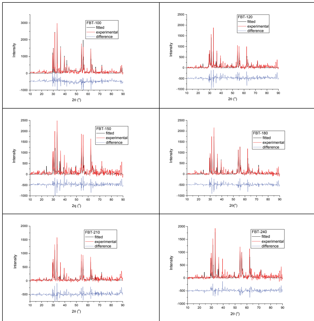
Figure S1. Rietveld analysis of XRD patterns of mechanically activated Fe:BaTiO 3 powder mixtures sintered at 1200°C.
