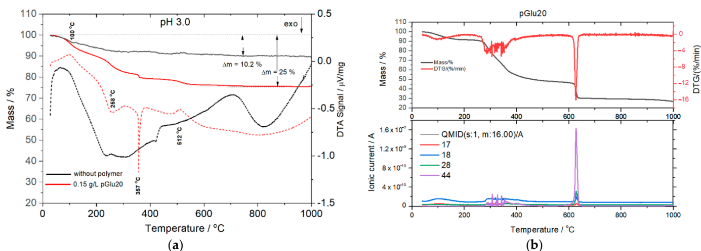
Figure 4. (a) TG/DTA curves of the materials drawn at pH 3.0 without the additive and in the presence of 0.15 g/L pGlu20 measured at 5 K/min up to 1000 °C in an air atmosphere. (b) TG/dTG-MS curves of pGlu20 powder at 5 K/min up to 1000 °C in an Ar-20%O 2 atmosphere.
