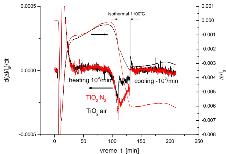
Fig.5. Dilatation and temperature of nano TiO 2 during the reheating a) and shrinkage rate b) as a function of time in two different atmospheres, air and nitrogen, of the previously sintered specimen at 1100°C.
