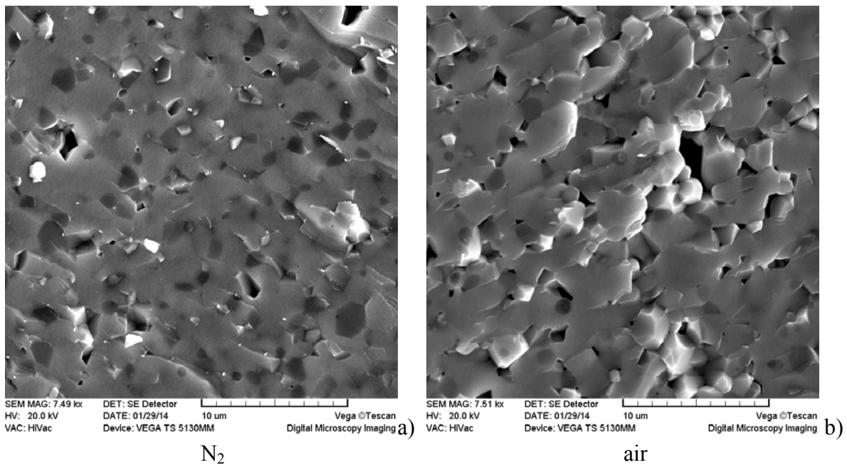
Fig.6. Scanning electron micrograph of TiO 2 nanopowder previously sintered and then a) reheated 1100°C 20 minutes, nitrogen atmosphere, b) reheated 1100°C 20 minutes, air atmosphere.
