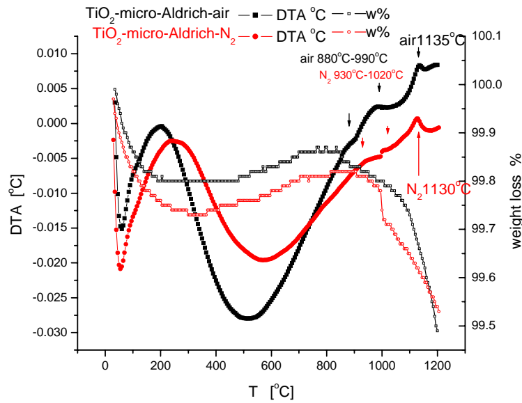
Fig.1. DTA of powders and TGA function of the a) TiO 2 nano and b) TiO 2 micro powders in nitrogen and air atmosphere.
