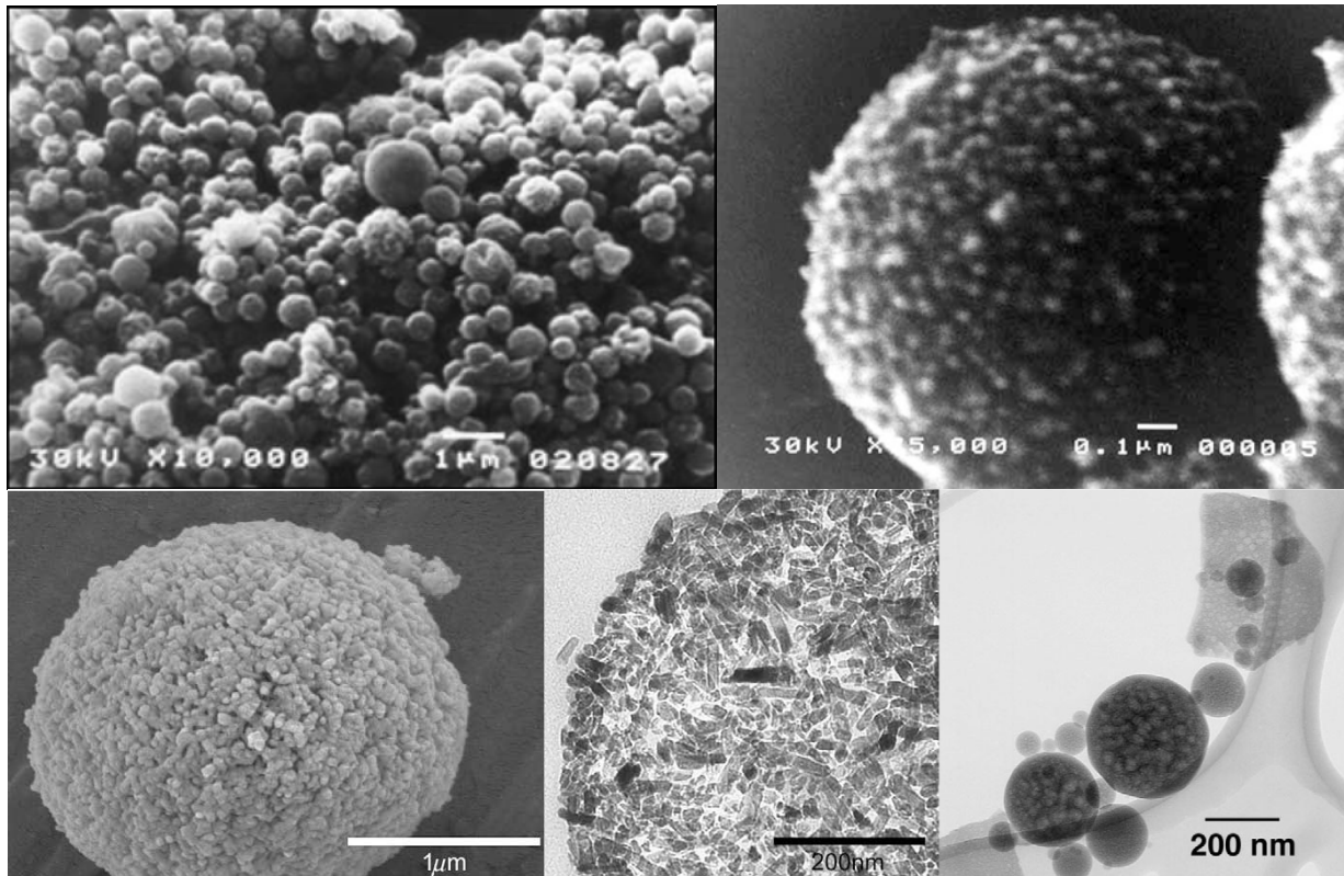
Fig.8. Uniform spherical HAP particles obtained using ultrasonic spray-pyrolytic processing (upper left), forming through aggregation of smaller spherical subunits (upper right). Reprinted with permission from Ref.189. Spray drying is another method that routinely leads to formation of microsized HAP particles through aggregation of nanosized subunits, and some of the morphologies are shown in images in the bottom row. Reprinted from Ref. 190.
