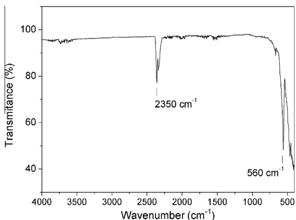
Fig. 5. FT-IR spectroscopy of nanocrystalline Y_{1.89}Yb_{0.1}Er_{0.01}O_3 powder annealed at 1100\text{ }^\circ\text{C} for 24 h.
