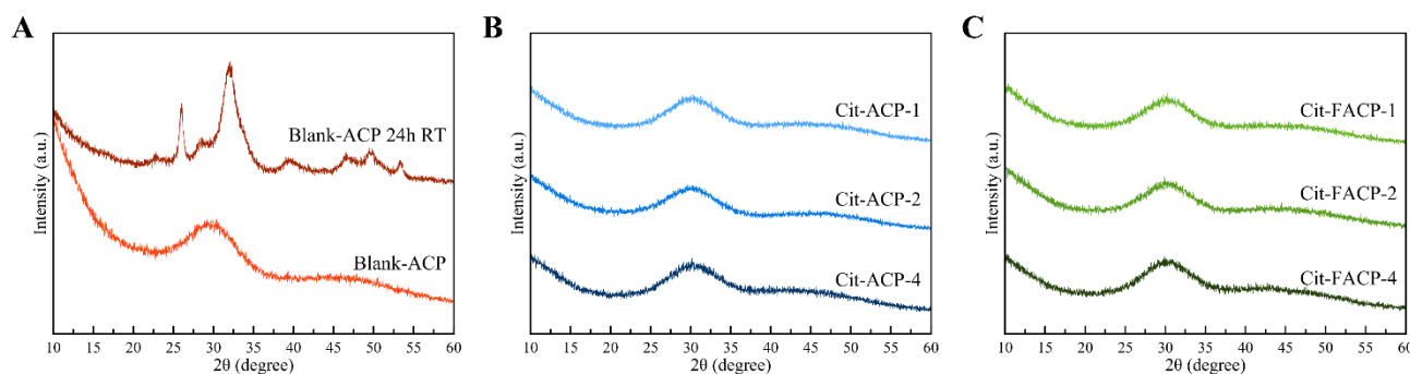
Figure 1. PXRD diffractograms of (A) Blank-ACP immediately after preparation and after 24 hours of storage at room temperature, (B) Cit-ACP and (C) Cit-FACP samples after 4 years of storage at room temperature.
