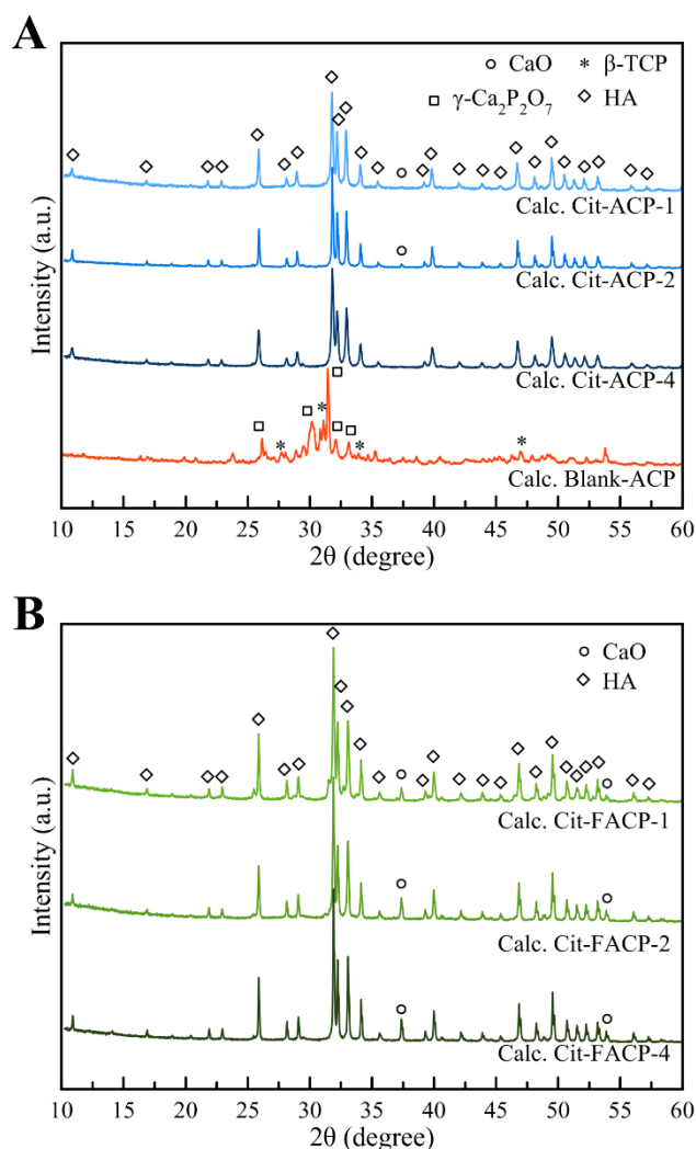
Figure 6. PXRD diffractograms of (A) calcined Blank-ACP, Cit-ACP-4, Cit-ACP-2, Cit-ACP-1, and (B) calcined Cit-FACP-4, Cit-FACP-2, and Cit-FACP-1.
