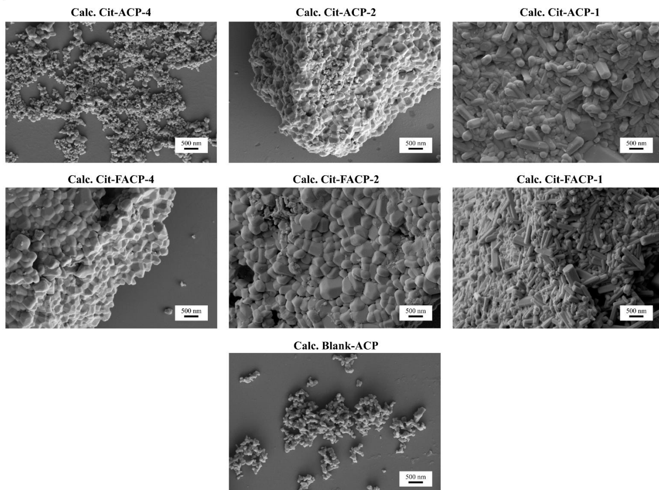
Figure 8. FEG-SEM micrographs of calcined samples.
