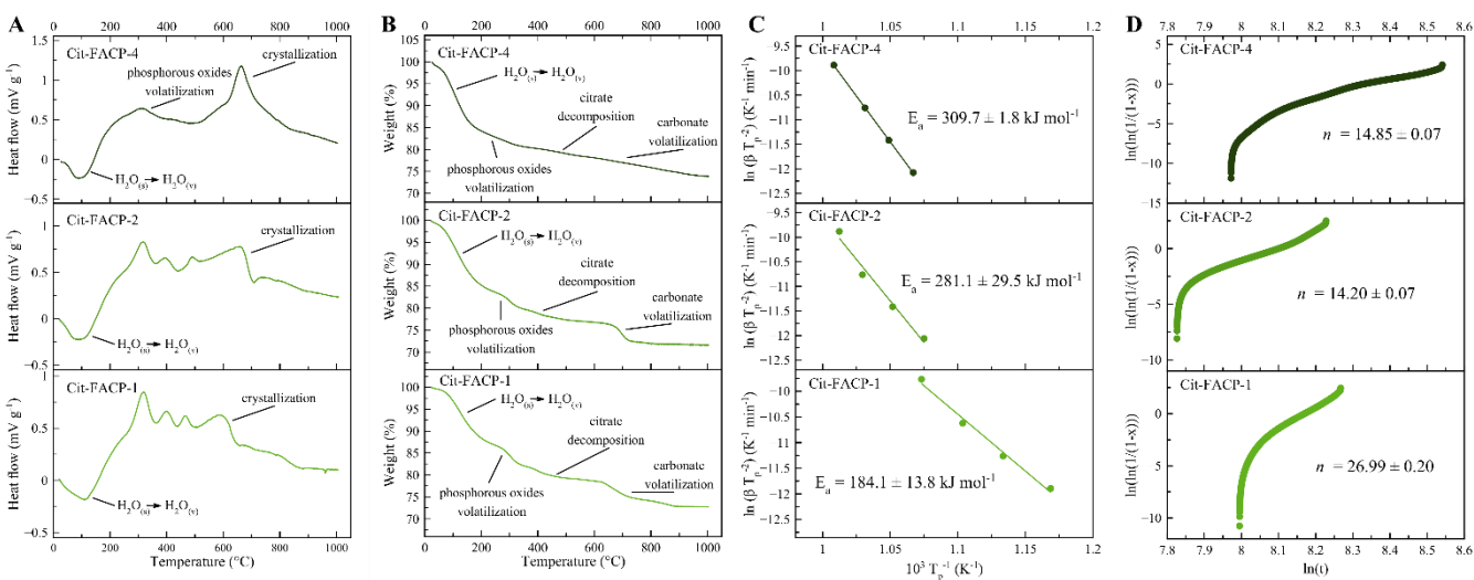
Figure 3. (A) DTA diagrams and (B) TGA curves obtained by heating Cit-FACP-4, Cit-FACP-2, and Cit-FACP-1 powders at the rate of 5 °C/min. (C) Kissinger plots with corresponding E_a values and (D) Johnson-Mehl-Avrami-Kolmogorov curves with corresponding Avrami exponents n calculated from DTA curves.
