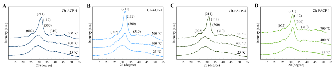
Figure 5. EDXRD diffractograms of (A) Cit-ACP-4, (B) Cit-ACP-1, (C) Cit-FACP-4, and (D) Cit-FACP-1 at 25 °C, 400 °C, and 700 °C.
