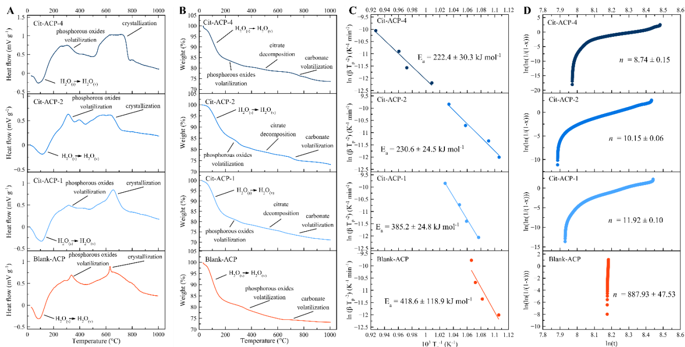
Figure 2. (A) DTA diagrams and (B) TGA curves obtained by heating Cit-ACP-4, Cit-ACP-2, Cit-ACP-1, and Blank-ACP powders at the rate of 5 °C/min. (C) Kissinger plots with corresponding E_a values and (D) Johnson-Mehl-Avrami-Kolmogorov curves with corresponding Avrami exponents n calculated from DTA curves.
