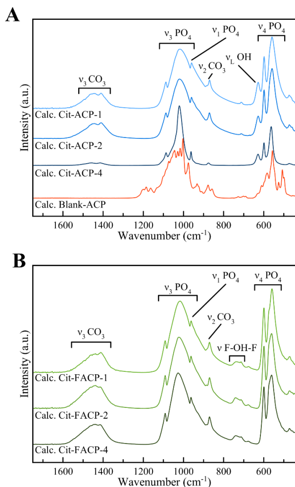
Figure 7. FT-IR spectra of (A) calcined Blank-ACP, Cit-ACP-4, Cit-ACP-2, Cit-ACP-1, and (B) calcined Cit-FACP-4, Cit-FACP-2, and Cit-FACP-1.
