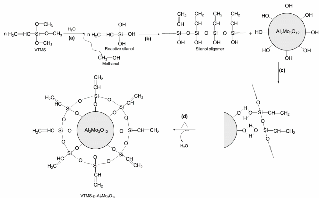
Fig.5 Scheme of (a) hydrolysis of VTMS; (b) oligomerization of reactive silanol molecules; (c) formation of hydrogen bonds between silanol oligomers and \text{Al}_2\text{Mo}_3\text{O}_{12} nanoparticles and (d) grafting of VTMS on \text{Al}_2\text{Mo}_3\text{O}_{12} surface through primary bonds
