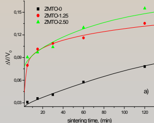
Cinc-titanate ceramics with MgO addition sintered isothermally at a) 1100°C and b) 1000°C
