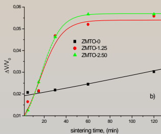
Cinc-titanate ceramics with MgO addition sintered isothermally at a) 1100°C and b) 1000°C
