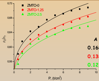
Ratio of relative density in dependence on the compaction pressure
