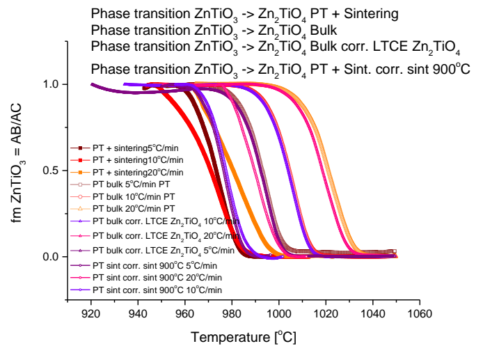
Fig 13. Phase transition kinetics comparison: Bulk and Sintered, Experimental vs. Corrected.
