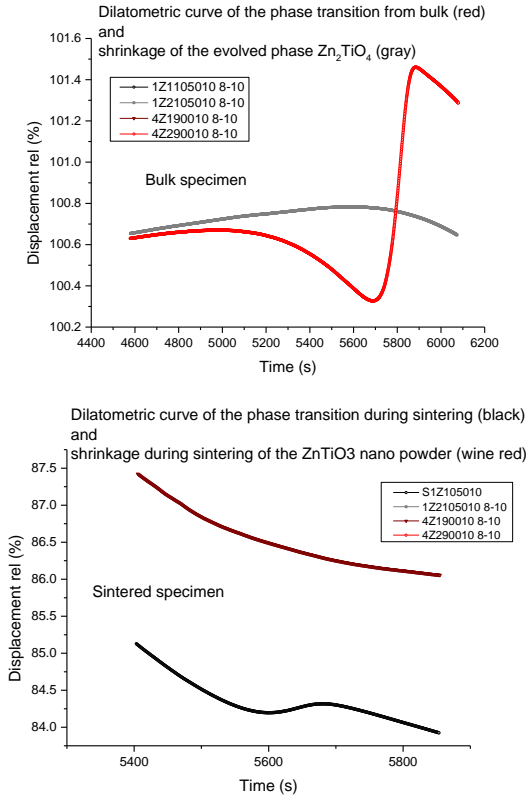
Fig 4. Dilatometric curves of phase transition ZnTiO 3 to Zn 2 TiO 4 extracted phase transition interval a) observed in a bulk specimen (red), thermal expansion of the Zn 2 TiO 4 phase (gray). b) Dilatometric curves of the phase transition and sintering (black), and sintering phenomenon without phase transition (wine red).
